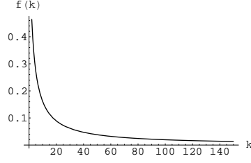
FIGURE 3. f(k) - k + 1 > 0 .
